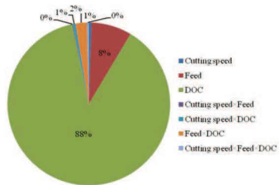
Fig. 1. Percentage Contribution for F_c
