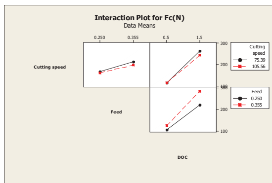
Fig. 7. Interaction plot for F_c
