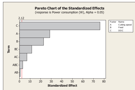
Fig. 4. Pareto chart for Power consumption
