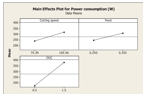
Fig. 6. Main effects plot for Power consumption
