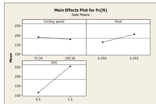
Fig. 5. Main effects plot for F_c
