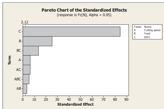
Fig. 3. Pareto chart for F_c
