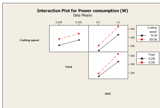
Fig. 8. Interaction plot for Power consumption
