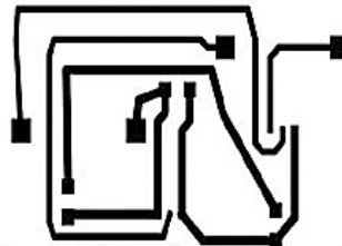
Figure 2: PCB layout of Music generator
