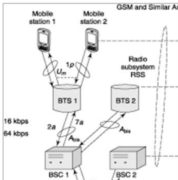
Figure 2. Connection interfaces in the RSS subsystem between BSC and the BTSs [1]
