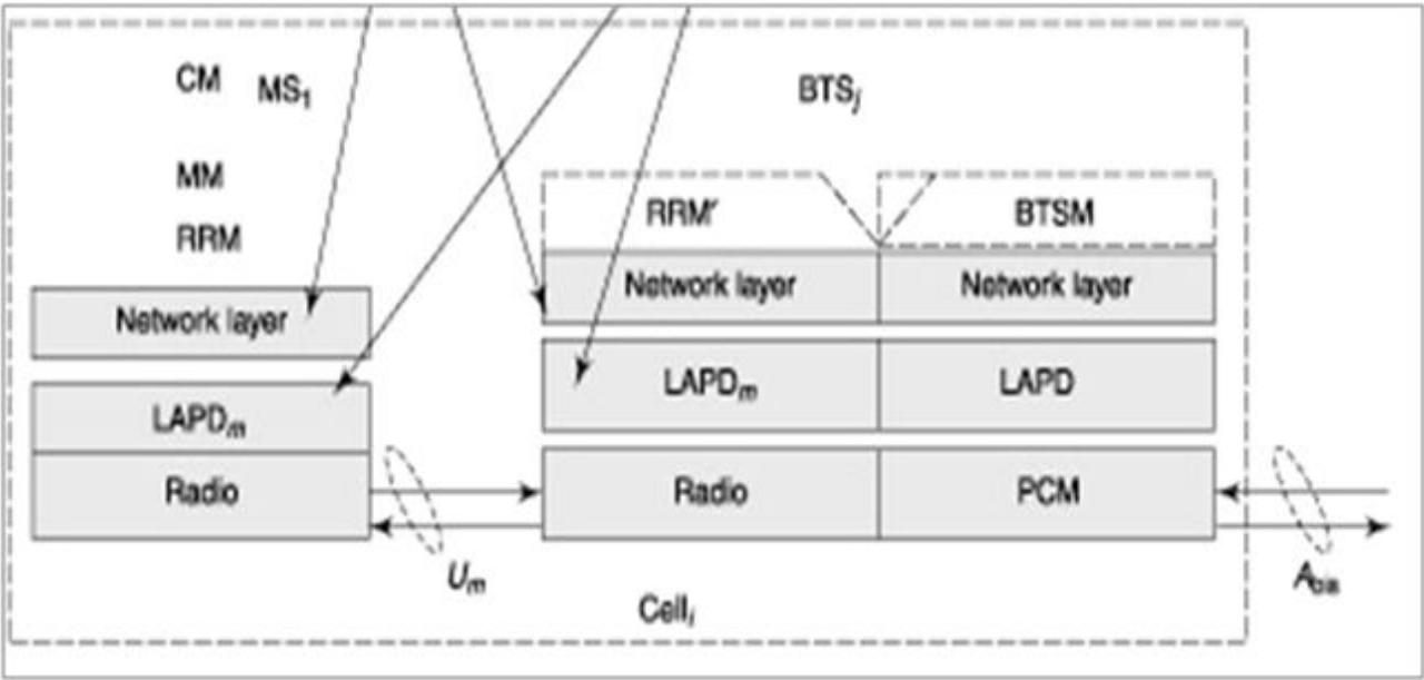
Figure 4. Protocol stack in GSM architecture
