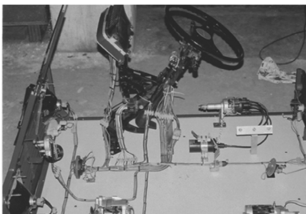
Fig.4 Cut Section Model of a Maruti Car Wiring
