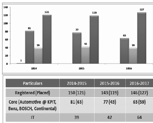
Fig 6.Placement Statistics
