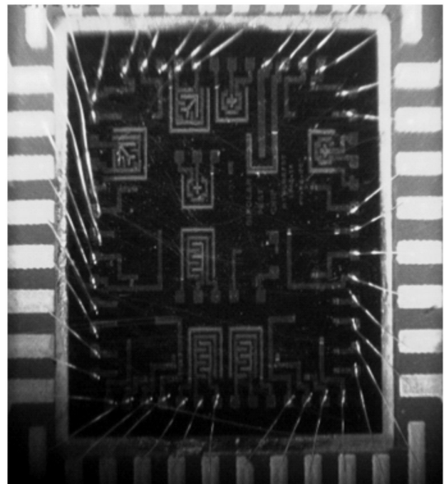
Fig. 4. MDC wire bonded to ceramic header
