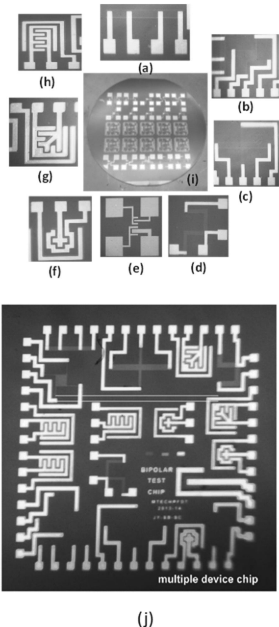
Fig. 2 Optical photograph of the fabricated wafer. (a) Bridge test structure, (b) Van der Pauw test structure, (c) Hall Effect test structure, (d) Kelvin cross bridge test structure, (e) Diodes, (f) – (h) bipolar transistors, (i) complete wafer with all structures and transistors, (j) multiple device chip
