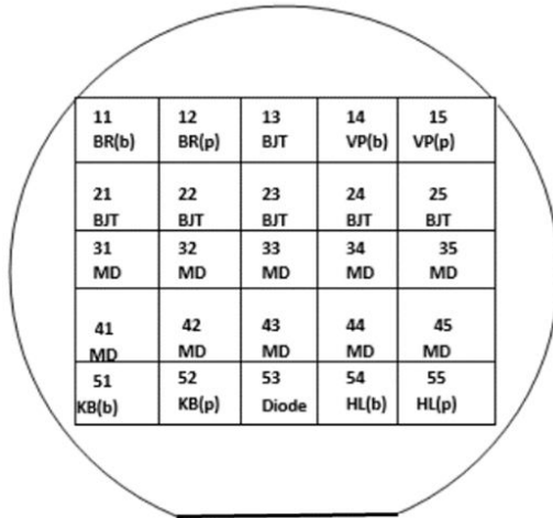
Fig. 1 Floor plan of the test chip. Chip No. 31-45 are identical chips having various test structures and devices for packaging on 40-pin header. Other chips contain single device or test structure: BR: Bridge test structure; VP: Van der Pauw test structure, KB: Kelvin Bridge test structure; HL: Hall Effect test structure; BJT: Bipolar junction transistor.
