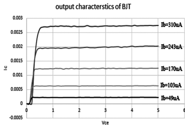
Fig. 3 Output characteristics of bipolar junction transistor in common emitter mode.
