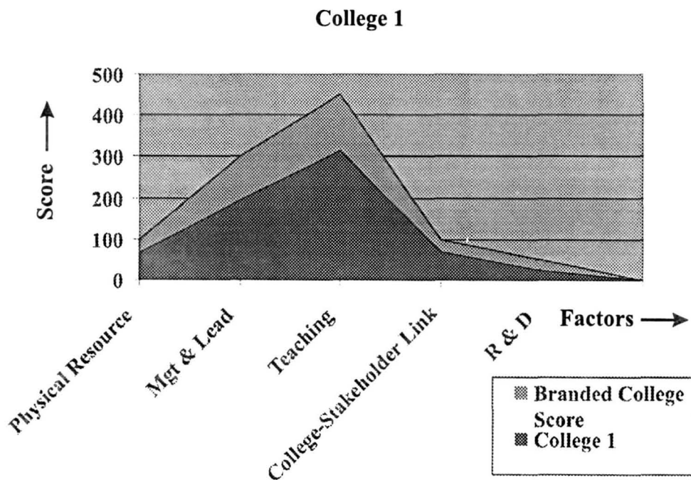
Figure 4: Area chart to show Factor wise score of college 1 with reference to branded college (refer Table 10)
