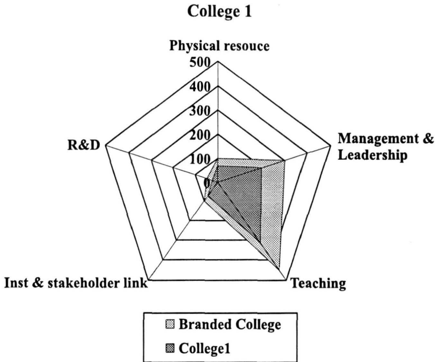
Figure 5: Radar diagram to show Factor wise score of college 1 with reference to branded college (refer Table 10)
